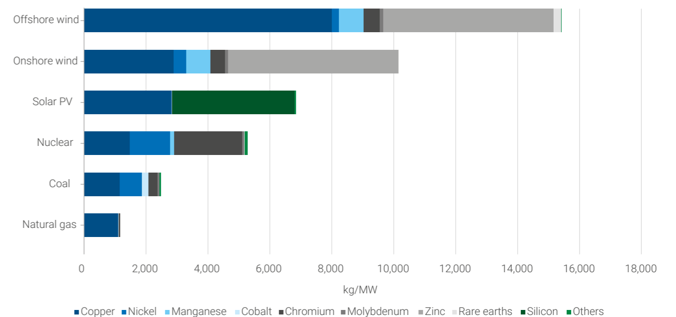
Figure 13: Mineral intensity of clean and conventional power generation technologies
